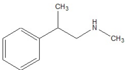
N-methylbetamethylphenethylamine
